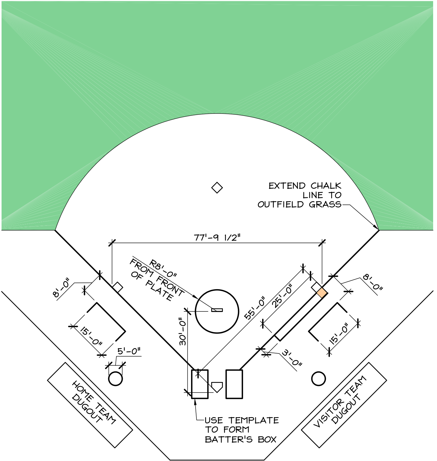
8 & UNDER FIELD SETUP
