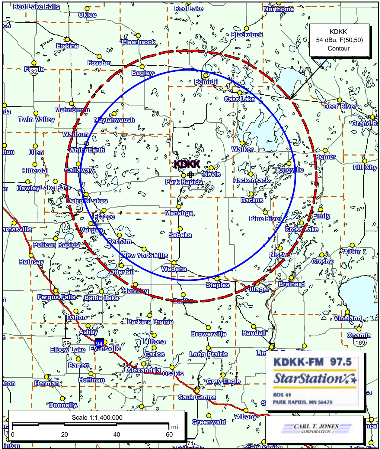
COVERAGE CONTOUR KDKK(FM) - PARK RAPIDS, MN CH. 248C1 (97.5 MHZ) - 100 KW ERP - 194 METERS HAAT
